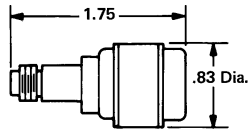
Model 55 SMA-F to N-M
